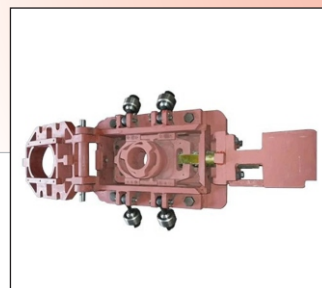
1QC Slide Gate Machine Assembly
