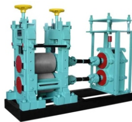
Pinch Rolls (A.C. / D.C.)
