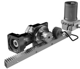
Lubricating Systems For Pinion & Reduction
